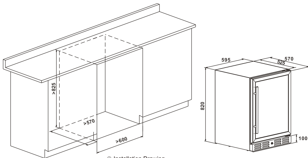
⊙ Installation Drawing
